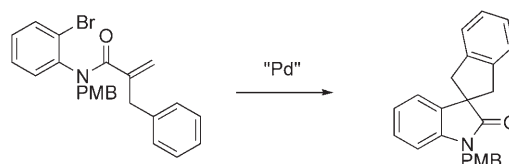
Scheme 1. Heck/C–H functionalization tandem reaction. PMB = p -methoxybenzyl.
